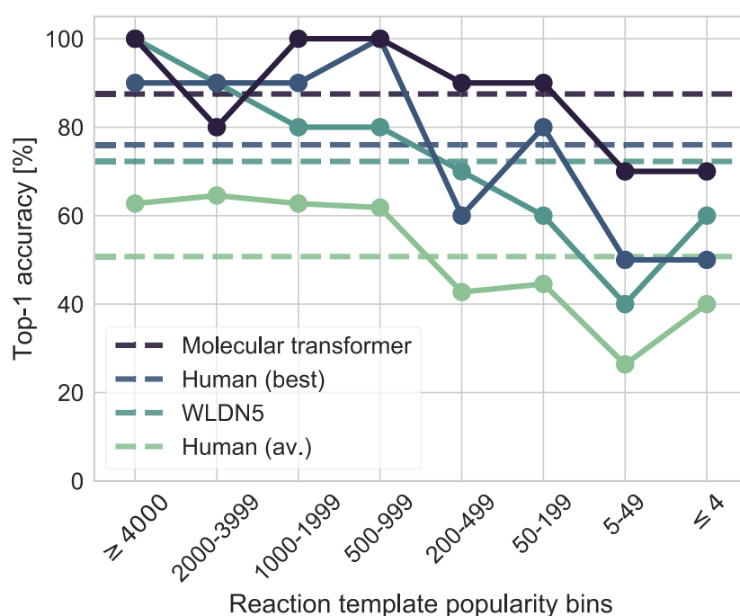
Figure 5. Top-1 accuracy of our model (mixed, USPTO_MIT) on 80 chemical reactions across eight reaction popularity bins in comparison with a human study and their graph-based model (WLDNS). 24
